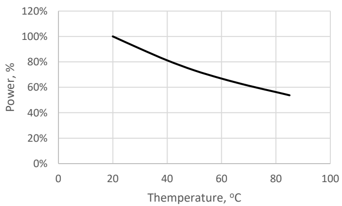
Fig 5. Relative Radiant Flux vs Ambient Temperature
