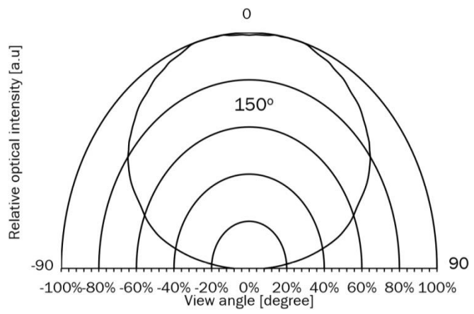
Fig 6. Far-field Emission Pattern
