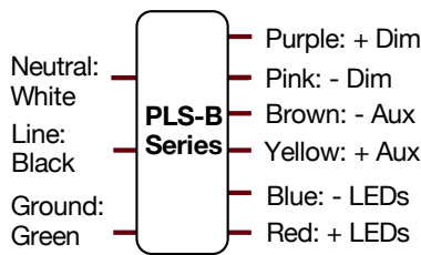
Wiring Diagram
