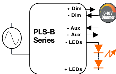
Application Diagram
